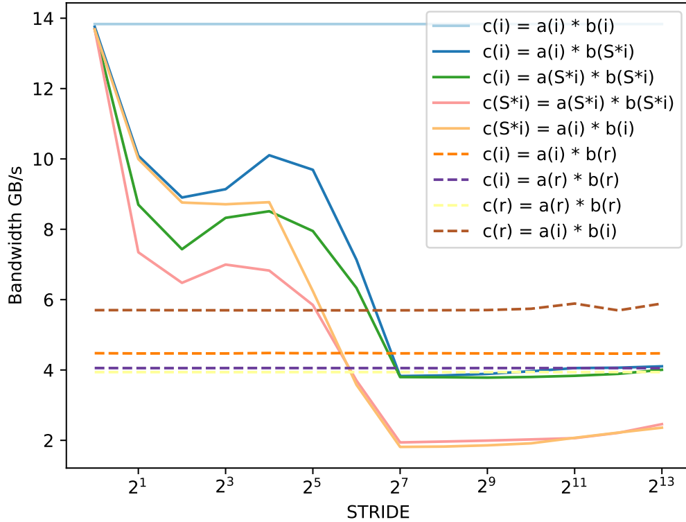
Figure 4.6: Bandwidth obtained for different access patterns using a single thread. Accesses labeled as x[i] represent sequential accesses, x[S*i] represent strided accesses, and x[r] represent random accesses.
